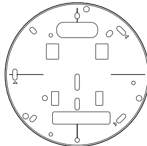
Mount plate
