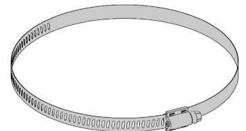
Large Pole Straps (2 pcs) Pole Diameter 84-152mm (3.3-6.0") Drive: 8mm Hex
